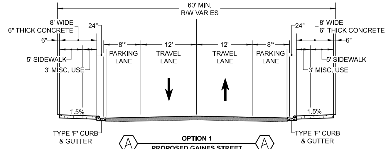
PROPOSED GAINES STREET MID-BLOCK PEDESTRIAN CROSSWALK
