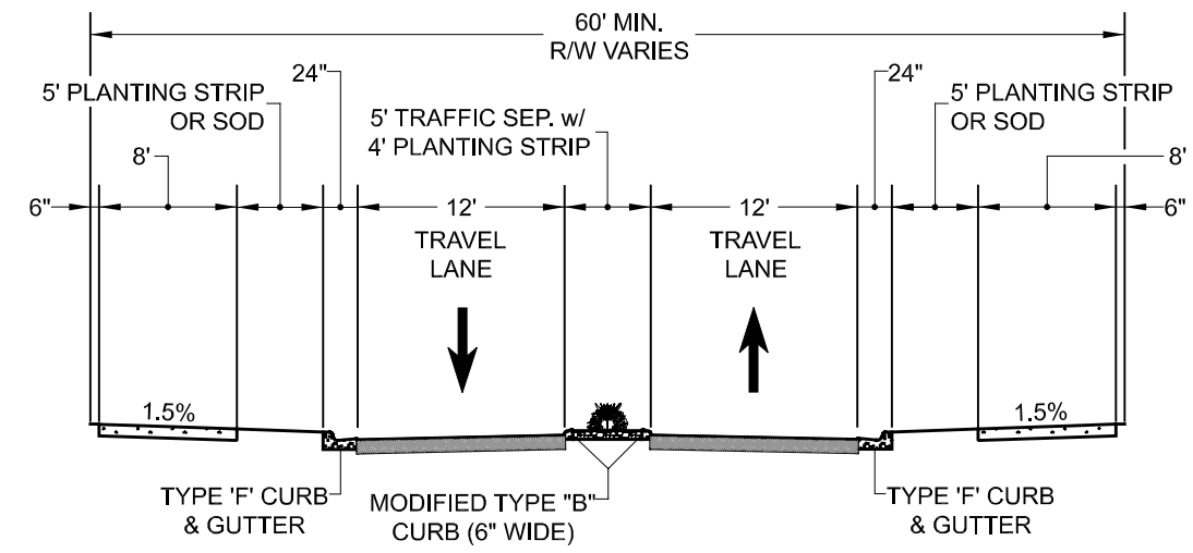
OPTION 1 PROPOSED GAINES STREET AT MID-BLOCK PEDESTRIAN CROSSWALK
